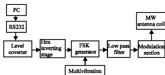
Fig. 2: Block diagram for trasmitter section of wireless modem
