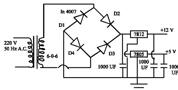
Fig. 6: Power supply
