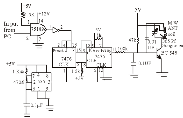
Fig. 5: Transmitter section
