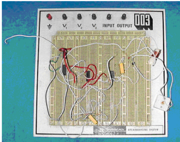
Photograph of transmitter section
