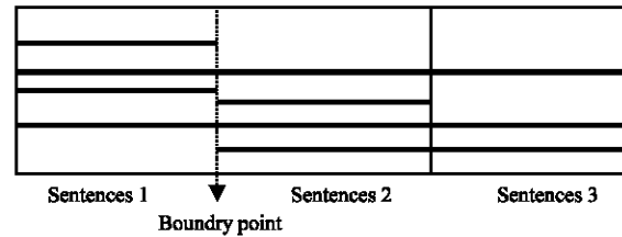
Fig. 1: Chain span schema with boundary point detected at end of sentence 1. w(n, n+1) values for each of these points are w(1, 2) = (2 \times 2) = 4 and w(2, 3) = (1 \times 0) = 0
