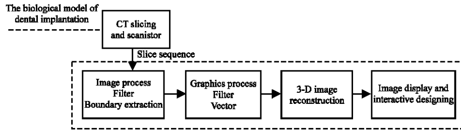
Fig. 1: CAD orientation system (processing module)
