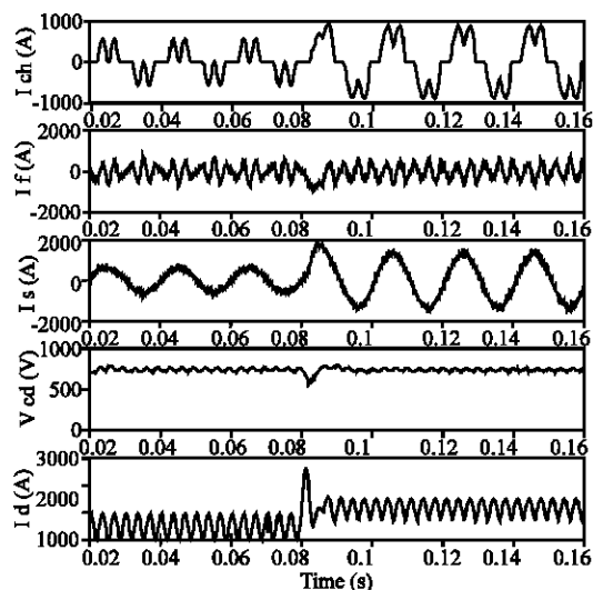
Fig. 8: Obtained waves for RC load
