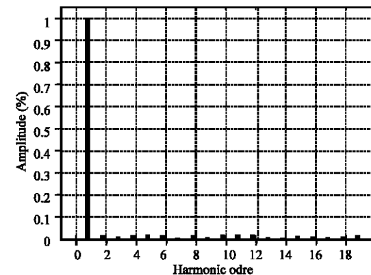
Fig. 7: Supply current spectrum with filter
