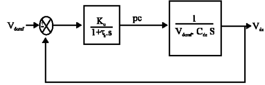
Fig. 3: DC voltage control block
