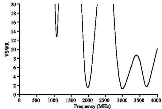
Fig. 4: Simulated 50 \Omega -VSWR vs. frequency
