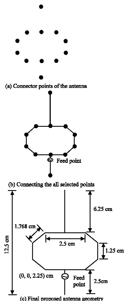
Fig. 1: Antenna geometry
