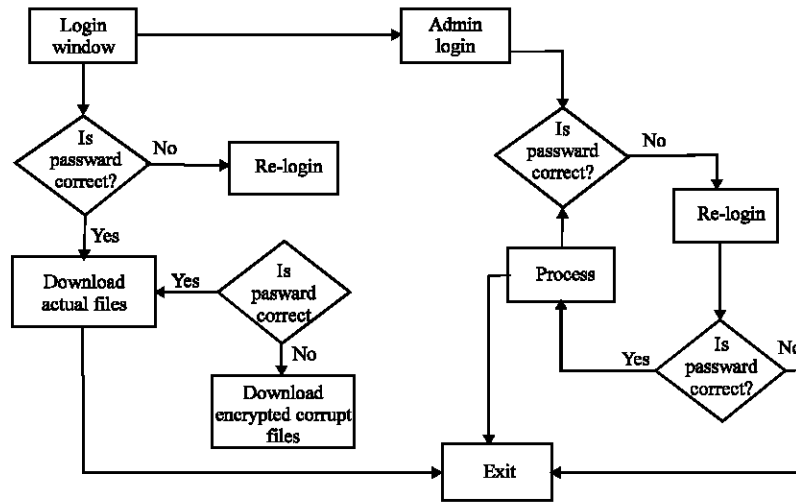
Fig. 1: Design application flowchart
