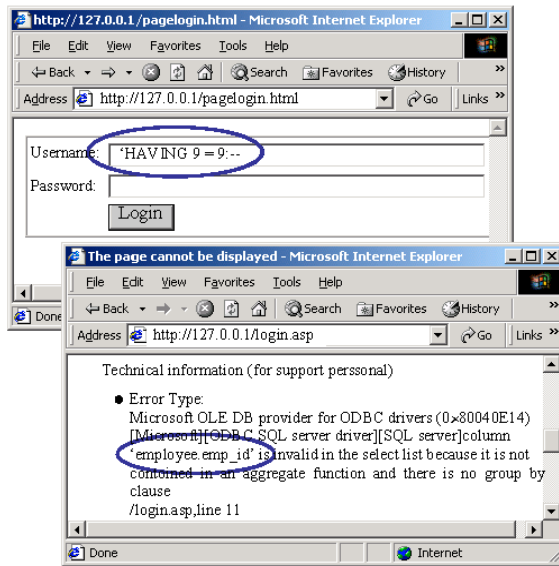
Fig. 4: Use HAVING command to get field name
