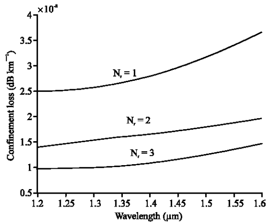
Fig. 10: Confinement loss of photonic crystal fiber against wavelength for different number of air hole rings. Air hole diameter, d = 5 \mu\text{m} and pitch \Lambda = 6.75 \mu\text{m}
