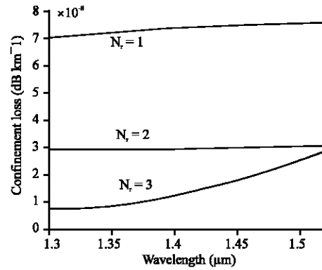
Fig. 12: Confinement loss of photonic crystal fiber against wavelength for different Number of air hole rings. d = 6 \mu\text{m} and \Lambda = 6.75 \mu\text{m}
