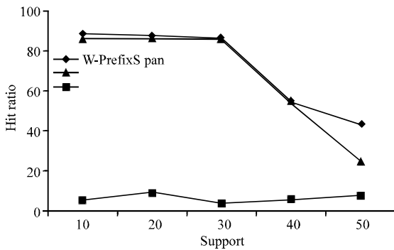
Fig. 5: Hit ratio
