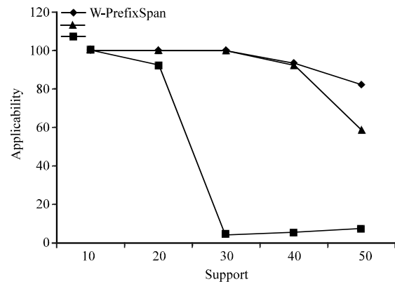
Fig. 4: Applicability
