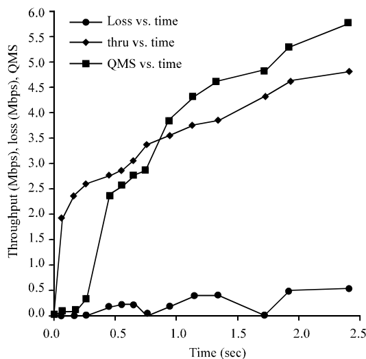
Fig. 12: Throughput-CMISHD vs. SASHA
