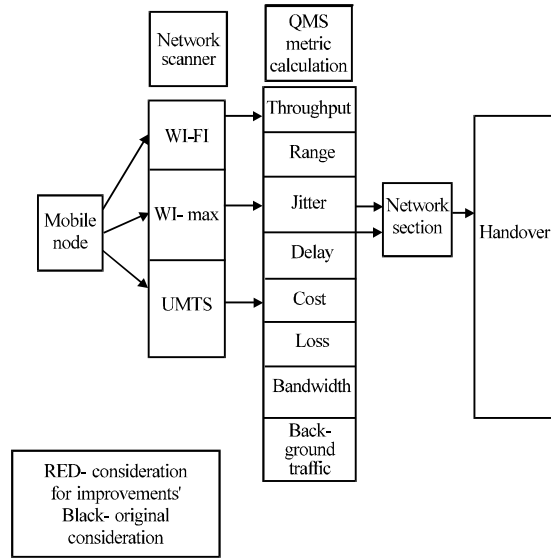
Fig. 2: CMISHD architecture
