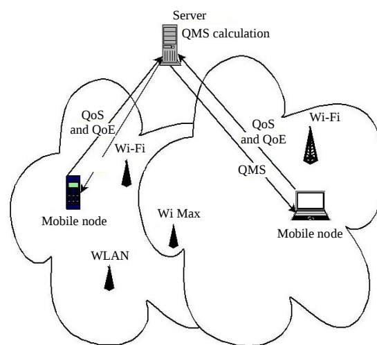
Fig. 1: CMISHD schematic
