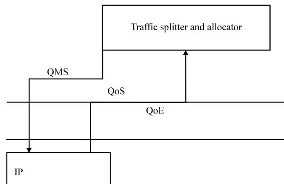
Fig. 8: Traffic splitter
