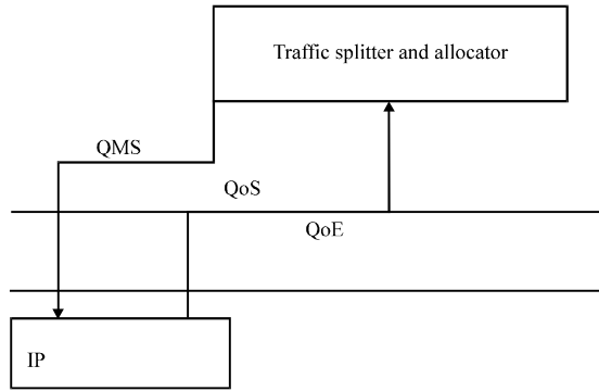
Fig. 9: QMS calculator
