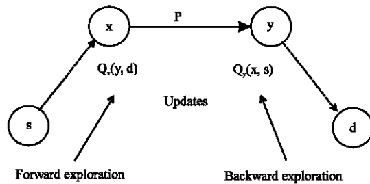
Fig. 5: Dual reinforcement Q Routing (DRQ Routing)
