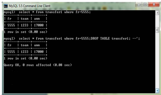
Fig. 3: Piggy-backed query
