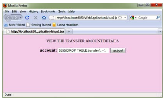
Fig. 12: Fund transfer details with Piggy backed injection
