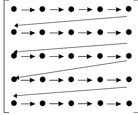
Fig. 7: Original image pixels comparison using Raster-Scan Method
