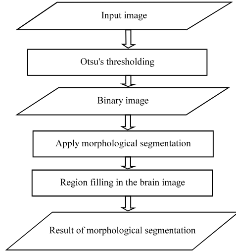
Fig. 2: The process flow of the proposed algorithm
