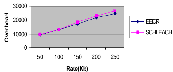
Fig. 16: Rate vs overhead
