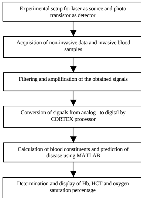
Fig. 1: Flow diagram of laser based system
