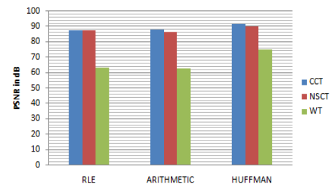
Fig. 12: Comparison of PSNR
