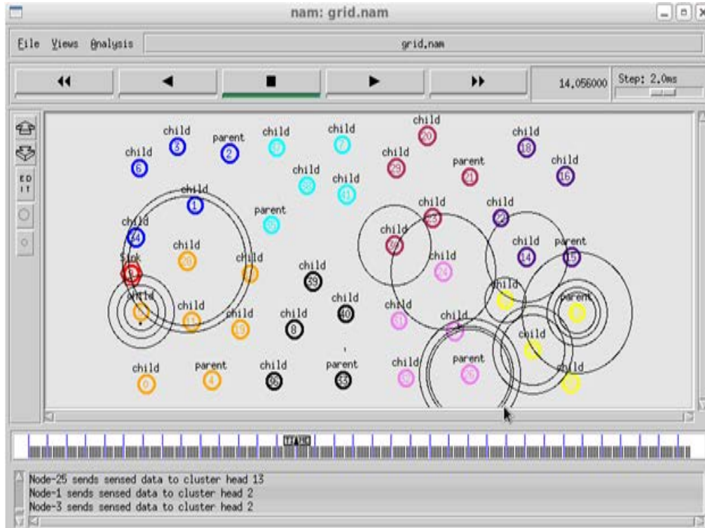
Fig. 3: Execution of ClusteredGSTEB in NAM window
