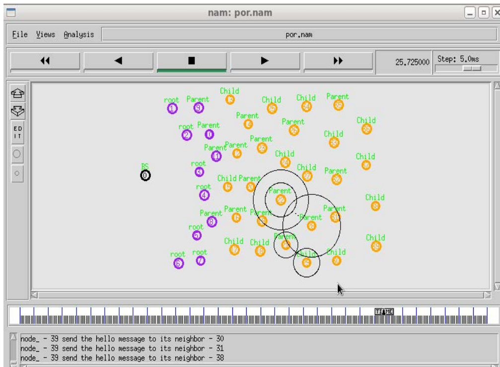
Fig. 4: Execution of GSTEB in NAM window
