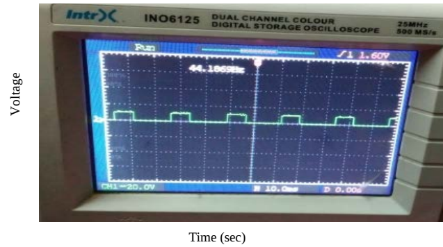
Fig. 17: Switching pulse from the PIC; X-Axis 1 unit = 1ms; Y-Axis 1 unit = 5v
