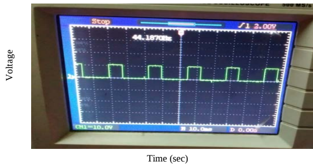
Fig. 18: Driver output for the switch M1; X-Axis 1 unit = 1ms; Y-Axis 1 unit = 10v
