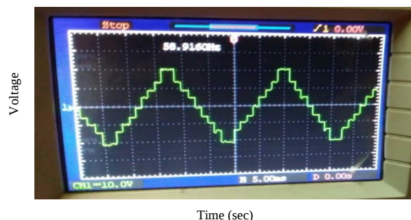
Fig. 21: Output voltage of the multi level inverter; X-Axis 1 unit = 1ms; Y-Axis 1 unit = 20 v
