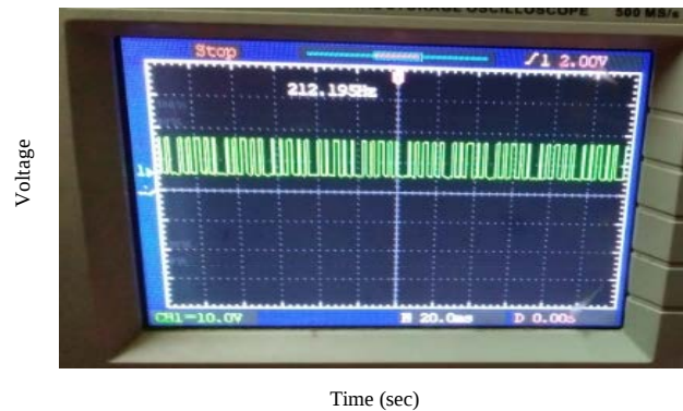
Fig. 20: Driver output for the device M3; X-Axis 1 unit = 1ms; Y-Axis 1 unit = 10v
