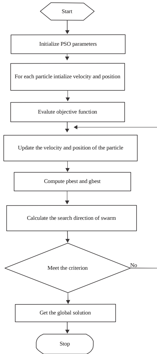
Fig. 2: PSO flowchart
