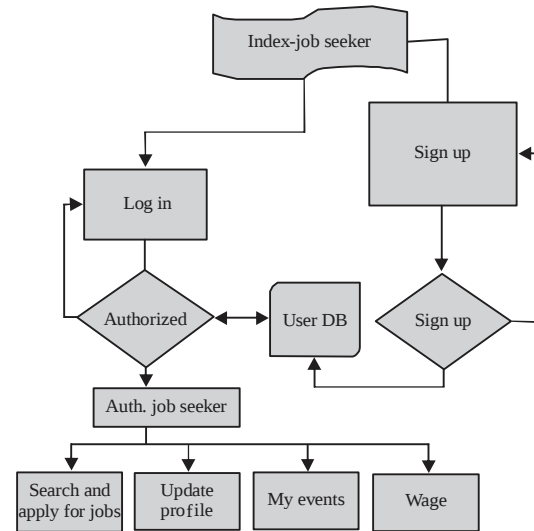
Fig. 1: Flowchart of the working principle
