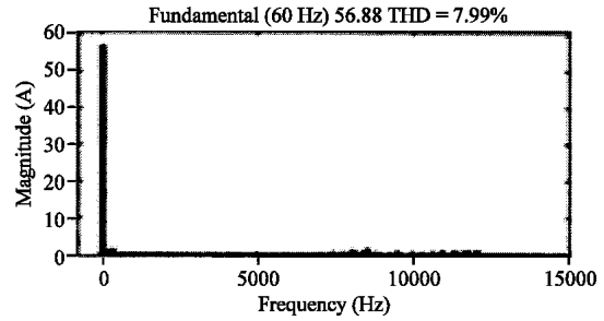
Fig. 9: Harmonic spectrum of supply current for conventional fixed band hysteresis control without interference phenomena
