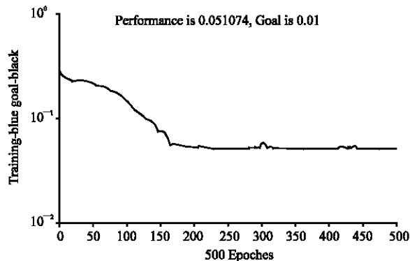
Fig. 9: Network training
