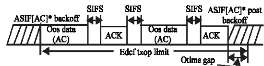
Fig. 4: CFB timing structure
