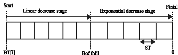
Fig. 5: Backoff time decrease phases
