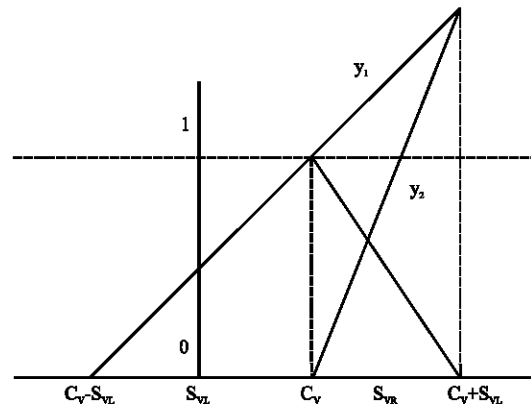
Fig. 4: Membership function
