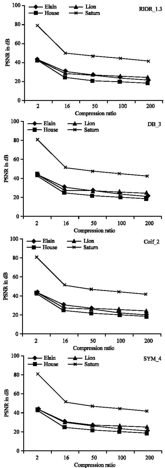
Fig. 5: Comparison of compression performance in terms of PSNR values with wavelets provides better results in their respective wavelet family on test image
