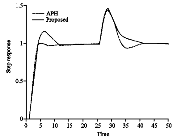
Fig. 6: Closed-loop step responses resulting from applying the proposed and APH methods to G_2(s)
