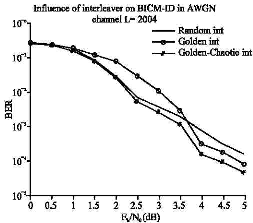
Fig. 4: Effect of interleaving methods on the performance of BICM-ID in AWGN channel. 4-state, rate-1/2 convolutional code, 8-PSK modulation with 1002 information bits per block
