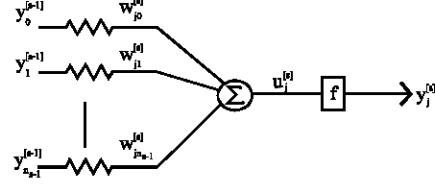
Fig. 1: A neuron j in a layer [s] of a MLP
