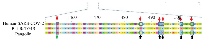
Fig. 1: Alignment of amino acids between 3 coronaviruses [4] . Red flags: Six similar amino acids between the coronavirus Pangolin and COVID-19; Black flags: Five different amino acids between coronavirus Bat-RaTG13 and COVID-19; Green flags: A similar amino acid between coronavirus Bat-RaTG13 and COVID-19
