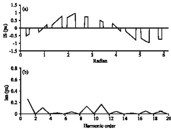
Fig. 3: The input current waveform in (pu), b: The harmonic spectrum of the input current
