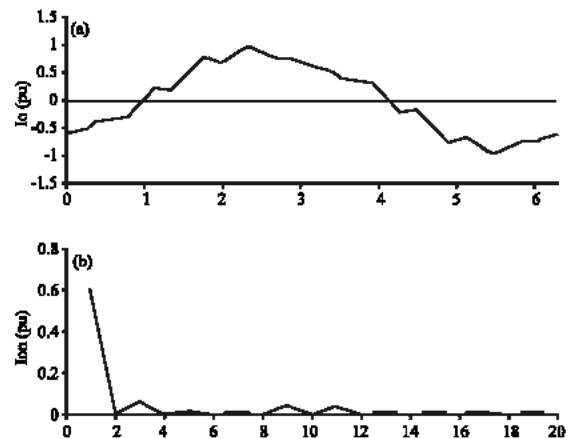
Fig. 5: The output current waveform in (p.u.) b: The harmonic spectrum of the output current waveform
