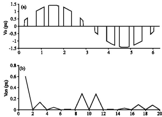
Fig. 6: The output voltage waveform in (p.u.), b: The harmonic spectrum of the output voltage
