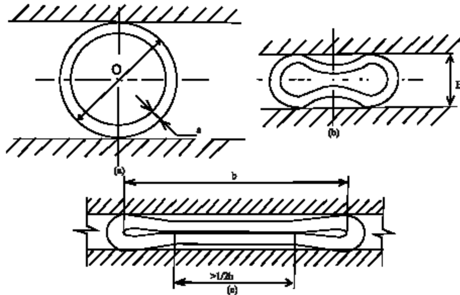
Fig. 1: Flattening test a-c
