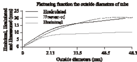
Fig. 7: Comparison of flattening minimum, calculated and measured in office the outside diameter before rolling and annealing
