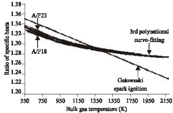
Fig. A2: Variation of the ratio of specific heats with respect to air-fuel ratio and temperature calculated by equilibrium program for gasoline HCCI engine data
