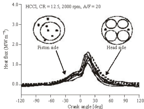
Fig. 8: Spatial variation of instantaneous local heat fluxes in a premixed HCCI engine
