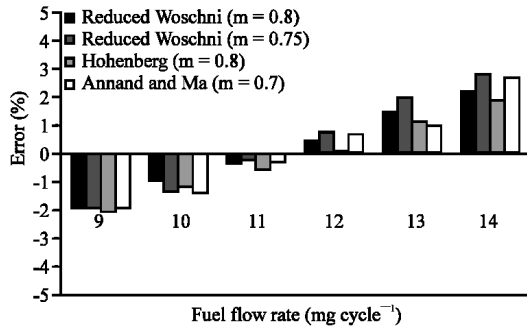
Fig. 15: Commulative gross heat release error associated with using selected heat transfer correlations over the range of loads
