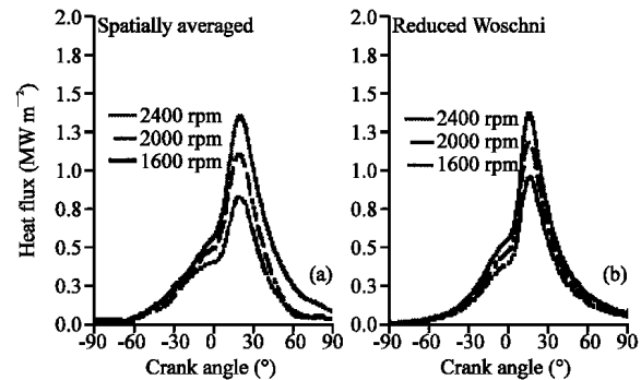
Fig. 20: Heat flux variation with speed: a) spatially-averaged measured and b) predicted heat flux using the new model given in Eq. 10
