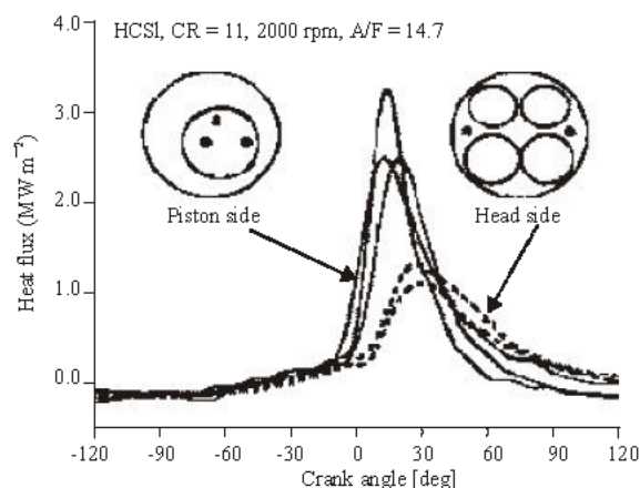
Fig. 7: Spatial variation of instantaneous local heat fluxes in a homogeneous charge spark ignition engine
