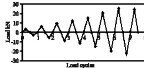
Fig 3a: Loading sequence for FCJS
