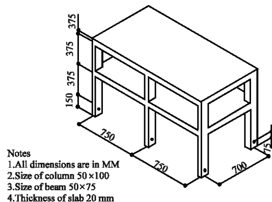
Fig. 1: Frame with slab
