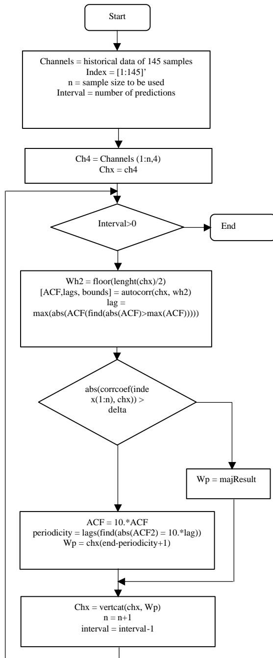
Fig. 7: Flowchart algorithm_3
