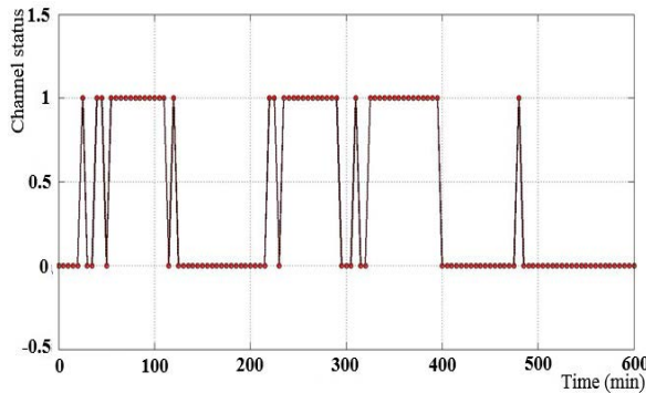
Fig. 14: Results for the interval of 101 samples
