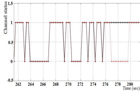
Fig. 23: Results for the interval of 951 samples using algorithms: 1 and 1-modified
