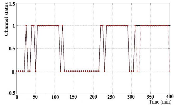
Fig. 18: Results for the interval of 61 samples
