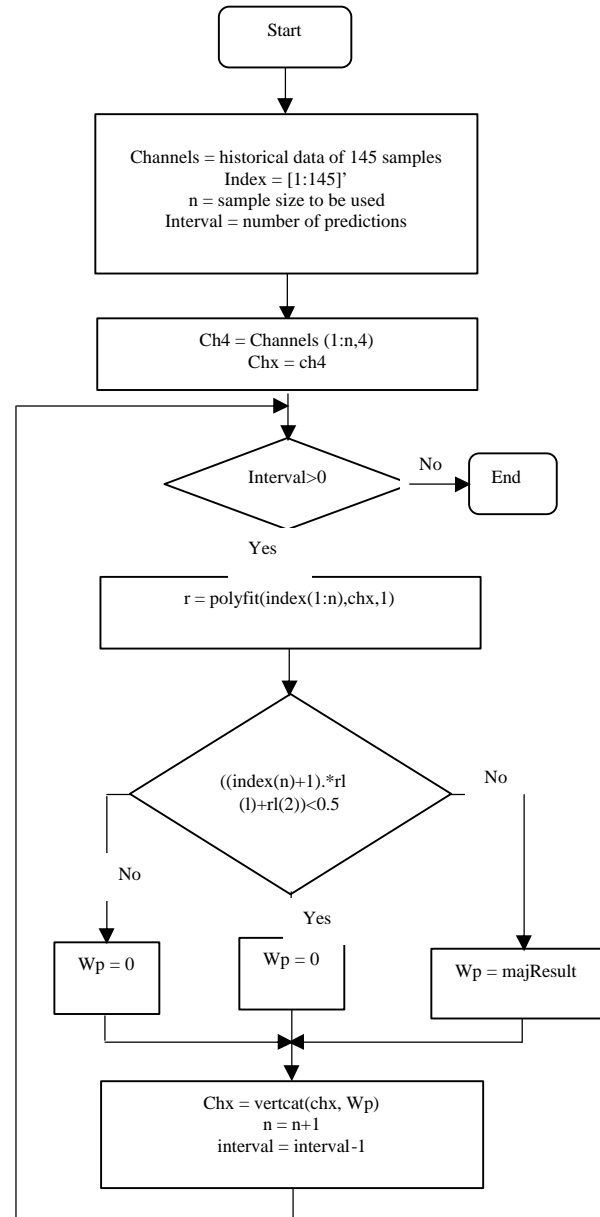
Fig. 6: Flowchart algorithm_6
