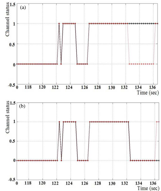
Fig. 20: a, b) Results for the interval of 451 samples using algorithms: 1 (Top) and 1-modified (Bottom)
