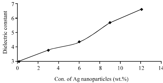
Fig. 7: Variation of dielectric constant with concentration of silver nanoparticles wt.% at 100 Hz for (PS-SPO-Ag) nanocomposites
