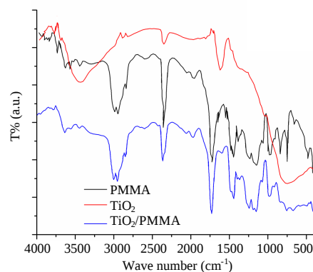
Fig. 1: FTIR spectra of PMMA polymer, anatase nanoparticles and TiO 2 /PMMA composite
