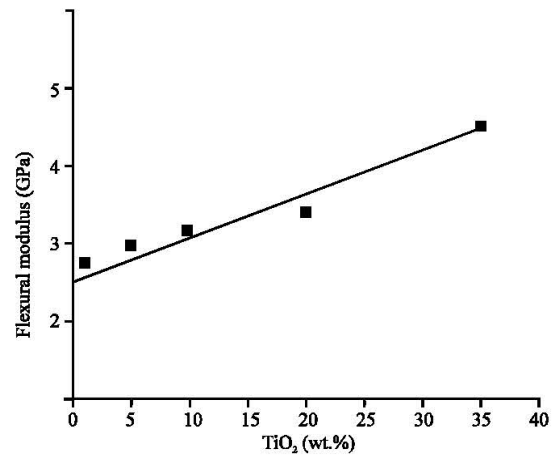
Fig. 7: The flexural modulus of elasticity of the \text{TiO}_2 /PMMA composites
