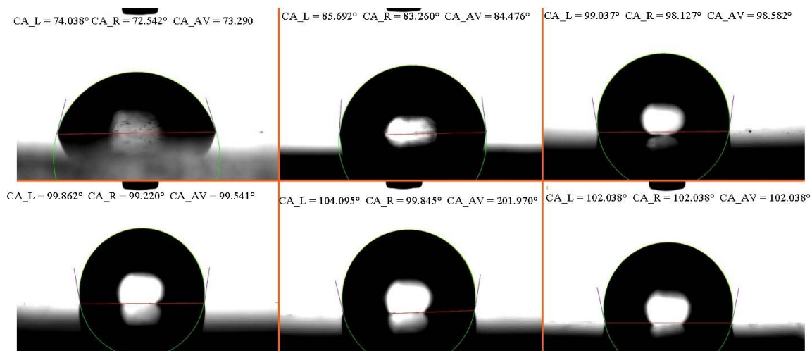
Fig. 8: The images of the sessile water drop on the surface of \text{TiO}_2 /PMMA composites
