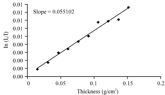
Fig. 9: Diagram between thickness in \text{g}/\text{cm}^2 and \ln I_0/I for energy 1330 keV
