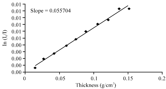
Fig. 7: Diagram between thickness in \text{g}/\text{cm}^2 and \ln I_0/I for energy 1170 keV
