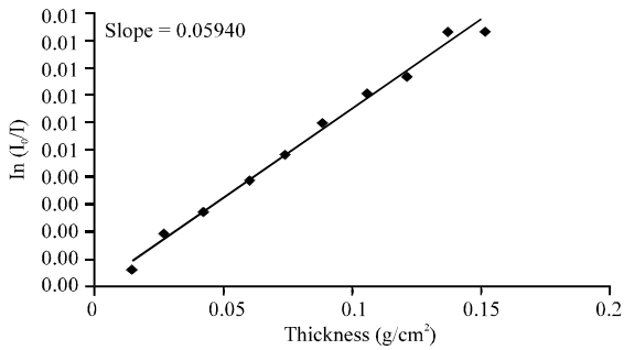
Fig. 8: Diagram between thickness in \text{g}/\text{cm}^2 and \ln I_0/I for energy 1275 keV
