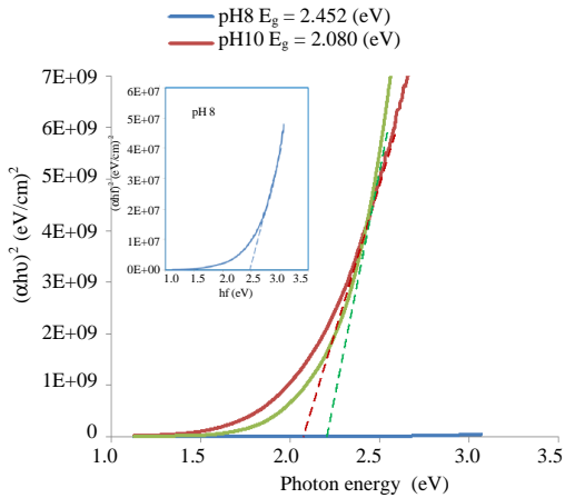
Fig. 8: Variation of (\alpha h\nu)^2 vs. h\nu of CuO thin films deposited at solution pH (8, 10 and 11.5)
