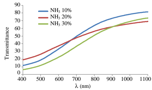
Fig. 5: Optical transmittance spectra of CuO films deposited at different ammonia concentration
