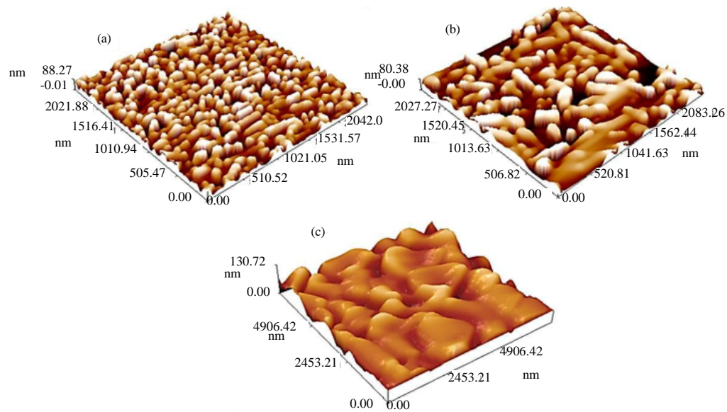
Fig. 3: AFM images of CuO thin films at different \text{NH}_3 ammonia concentration; a) 10%; b) 20% and c) 30%
