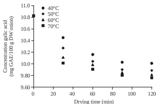
Fig. 3: Degradation of gallic acid (mg GAE/100 g DW onion) during heating at 40, 50, 60 and 70°C
