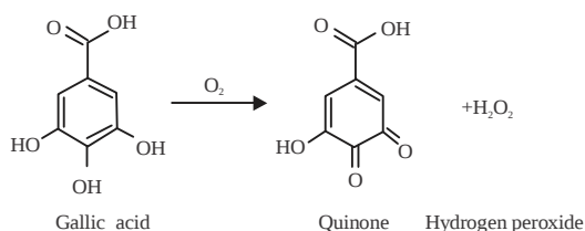
Fig. 4: Reaction of gallic acid thermal degradation [20]
