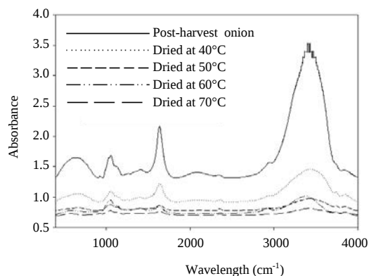
Fig. 5: FTIR spectra of fresh and dried onion at frequency of 400-4000 \text{cm}^{-1}
