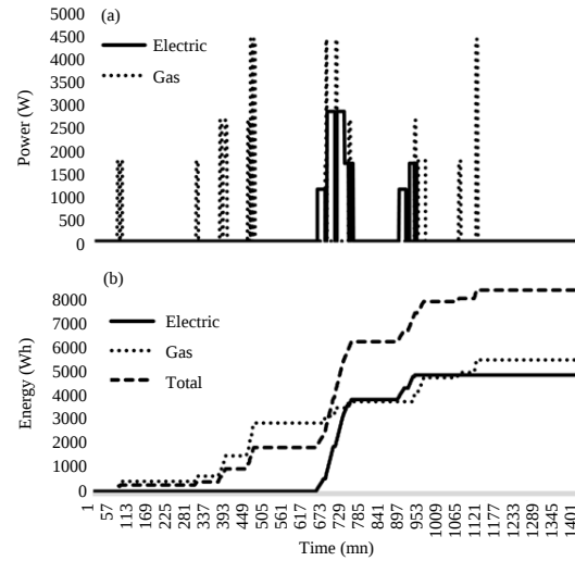
Fig. 4(a, b): Cooking equipment consumption related to EGE availability
