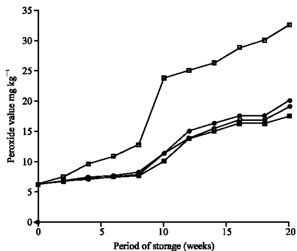
Fig. 1: Variation of peroxide value with period of storage (in weeks) for the palm oil samples. Open square (Sample A), solid square (Sample B), open circle (Sample C) and closed circle (Sample D)
