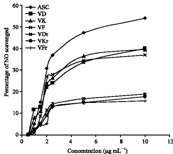
Fig. 3: Nitric Oxide (NO) scavenging activity of methanolic extracts of the three Vitex fruits and ascorbic acid
