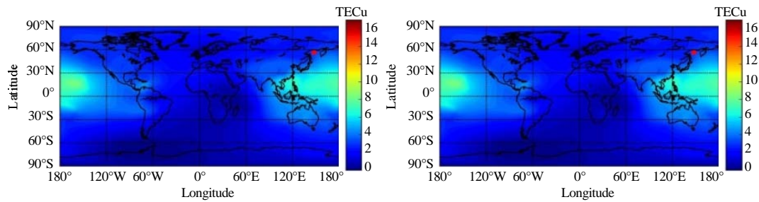
Fig. 1: The GIMs during the time period from 02:20-02:35 on 14 August, 2012 (UTC). The red spot in each GIM represents the location of the earthquake epicenter
