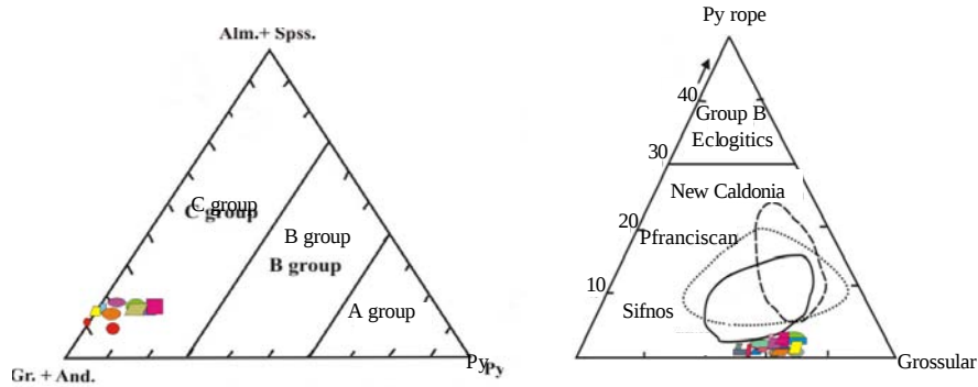
Fig. 4: Index diagram of skarn garnets in southwest of Dezg (Derived from
