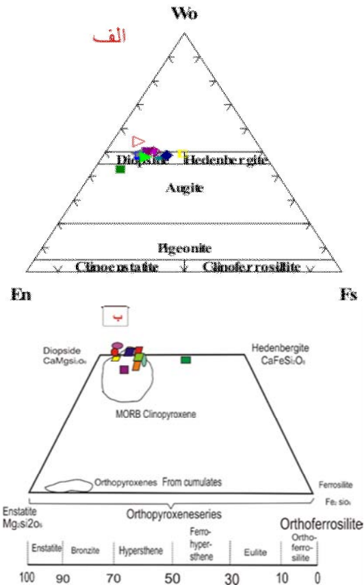
Fig. 6: a) Variations of clinopyroxene composition in skarn samples existing in southeast of Dezg; b) Quadrilateral chart of pyroxenes which indicate the presence of diopside and augite diopside in skarn samples
