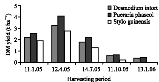
Fig. 1: Persistence of species under frequent harvesting
