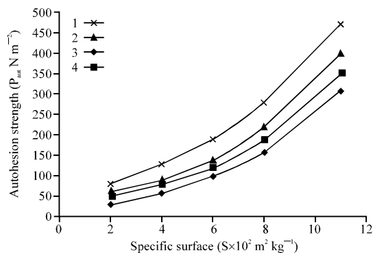
Fig. 2: Dependence of autohesion strength P_{aut} , H \cdot m^{-2} of dry mixes on specific surface S , m^2 \cdot kg^{-1} : 1) chalk+clay; 2) limestone+clay; 3) limestone+slag; 4) marl
